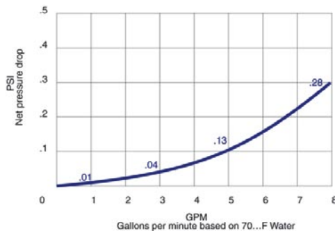
Pressure/Flow Chart
