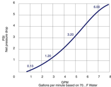
Pressure/Flow Chart
